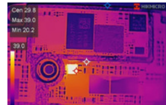
PCB
